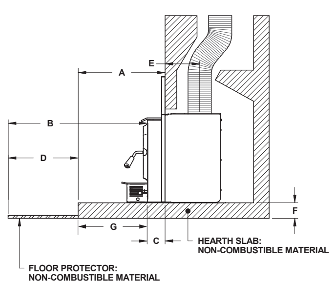
Figure 23: Additional Floor Protection - Raised Installation
