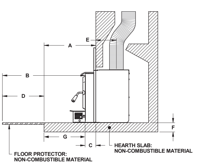
Figure 24: Additional Floor Protection - Not Raised Installation
