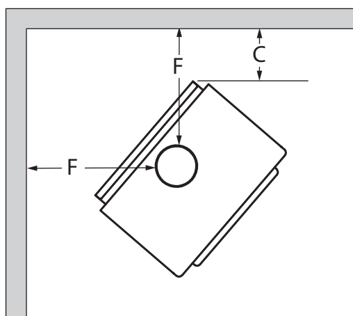
Figure 28: Clearances - Corner
