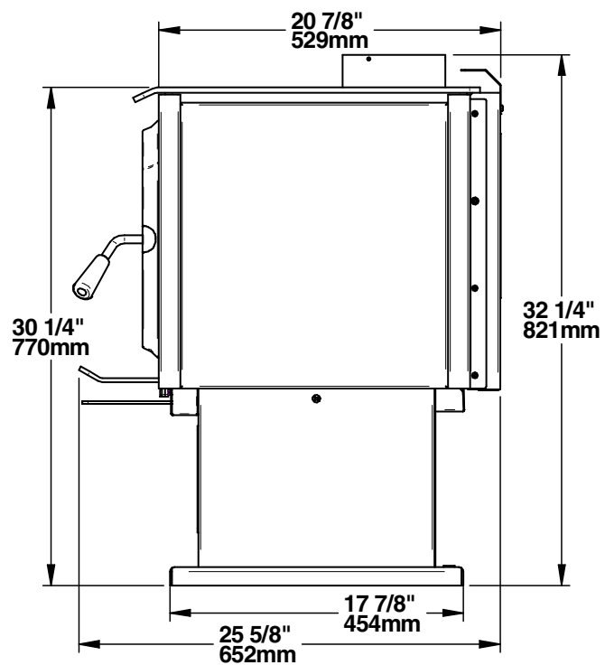
Figure 9: Side View
