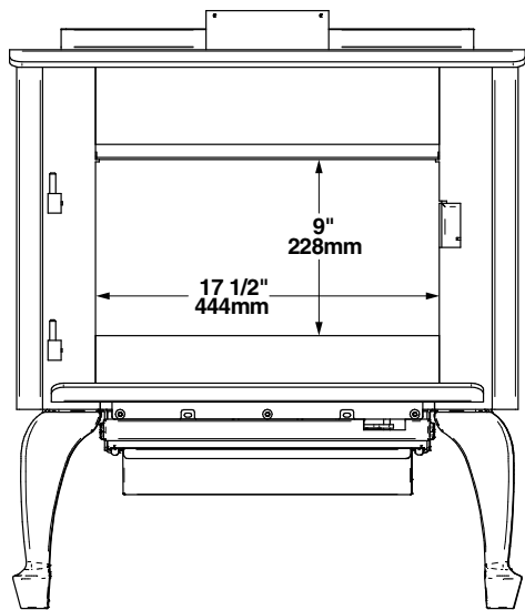
Figure 10: Door Opening
