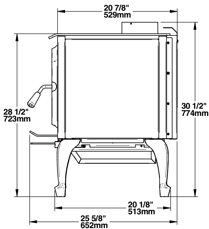
Figure 3: Side View
