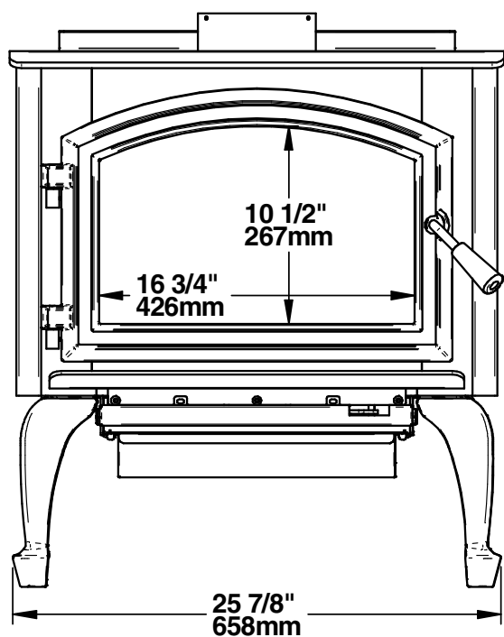
Figure 2: Front View
