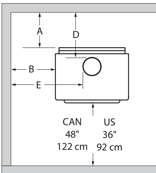
Figure 27: Clearances - Top
