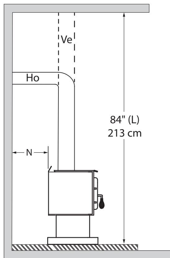
Figure 29: Clearances - Side
