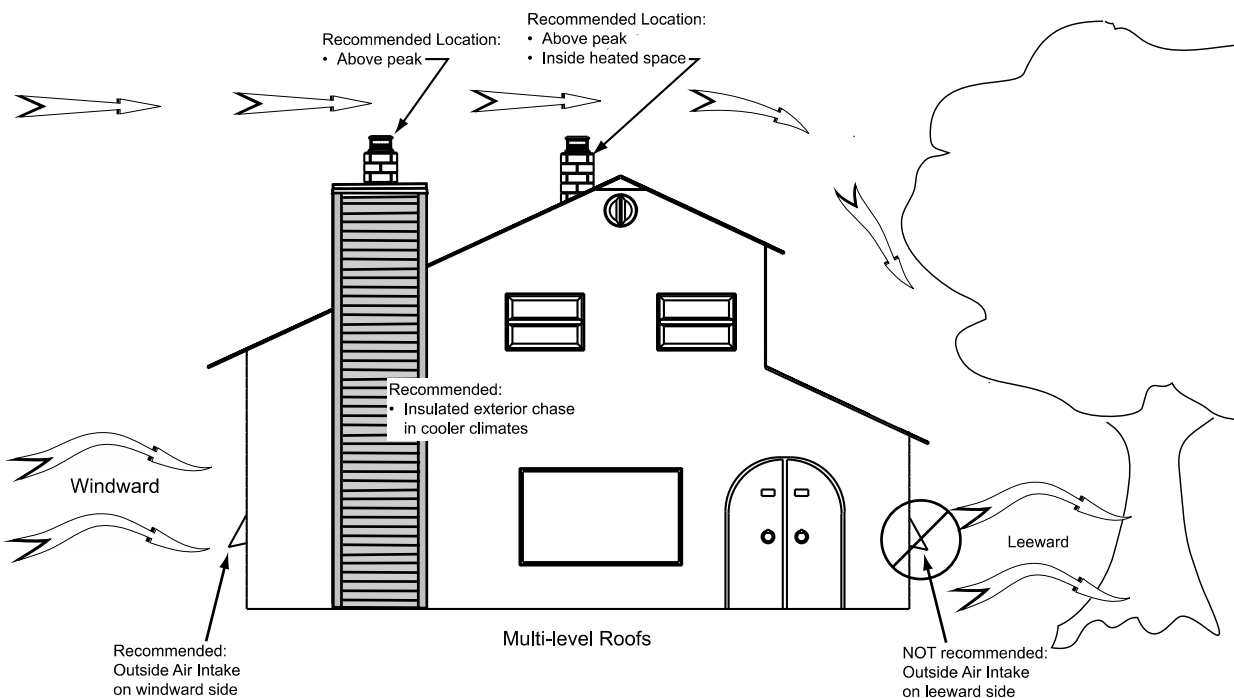
Figure 32: Air supply in conventional houses
