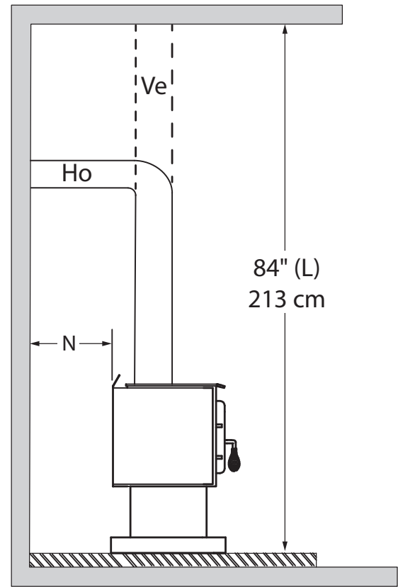
Figure 15: Clearances - Side
