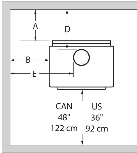
Figure 16: Clearances - Top
