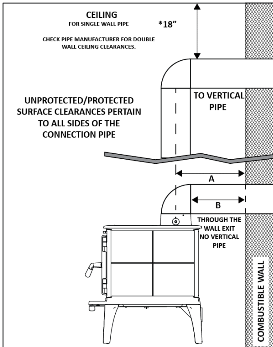
Figure 8: Chimney Connector Clearances to Combustibles
