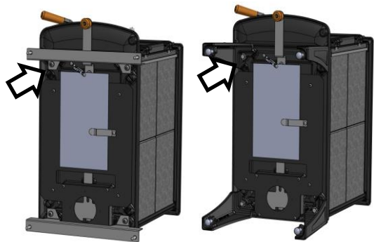
Figure 3 – Bracket Removal
