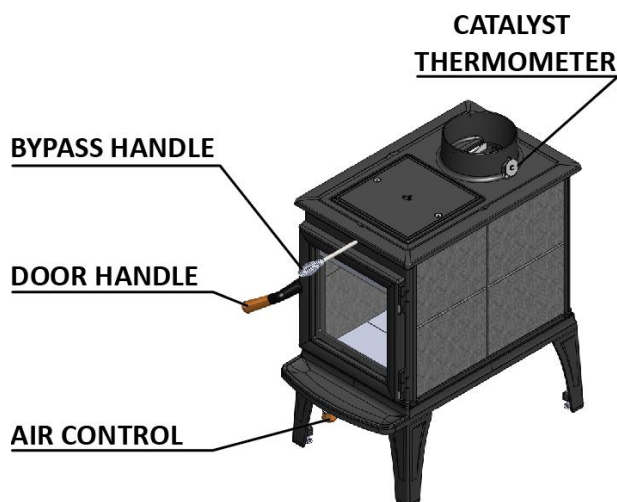
Figure 14 - Controls & Features
