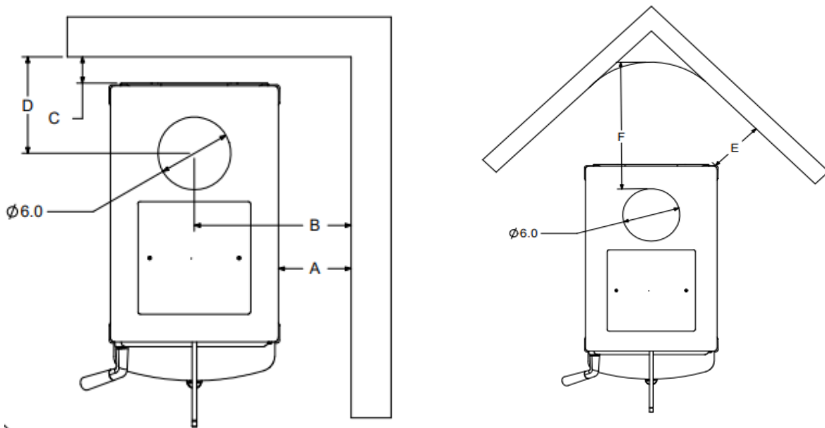
Figure 6 – Clearance to Combustibles
