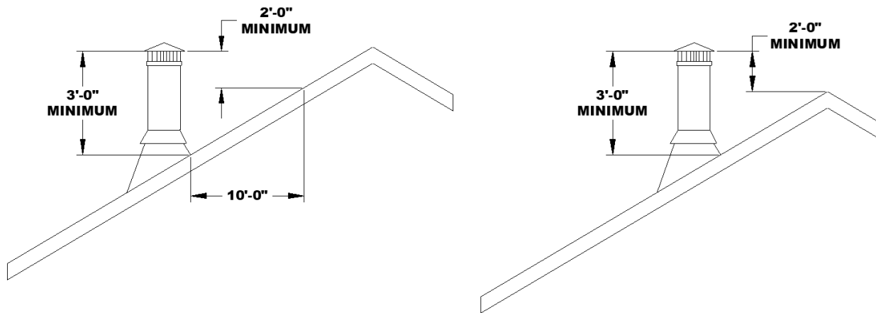
Figure 10 - Chimney Height Requirements
