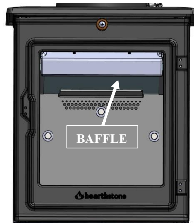
Figure 18 – Baffle Location
