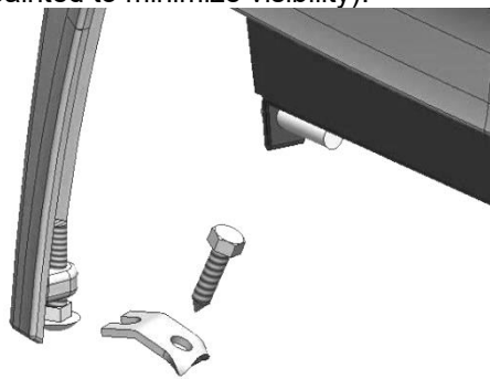
Figure 12 - Lock Down Detail
