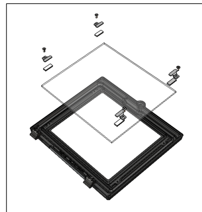
Figure 21 – Door Glass Kit
