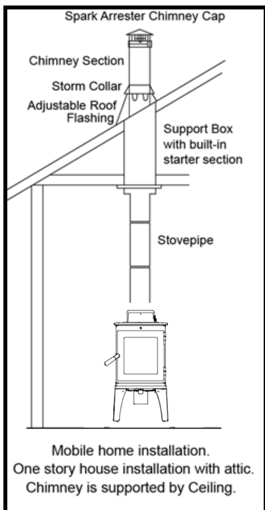
Figure 13 - Mobile Home Installation
