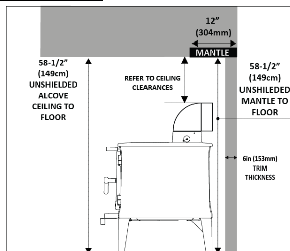
Figure 7 trim, mantle, and alcove clearances
