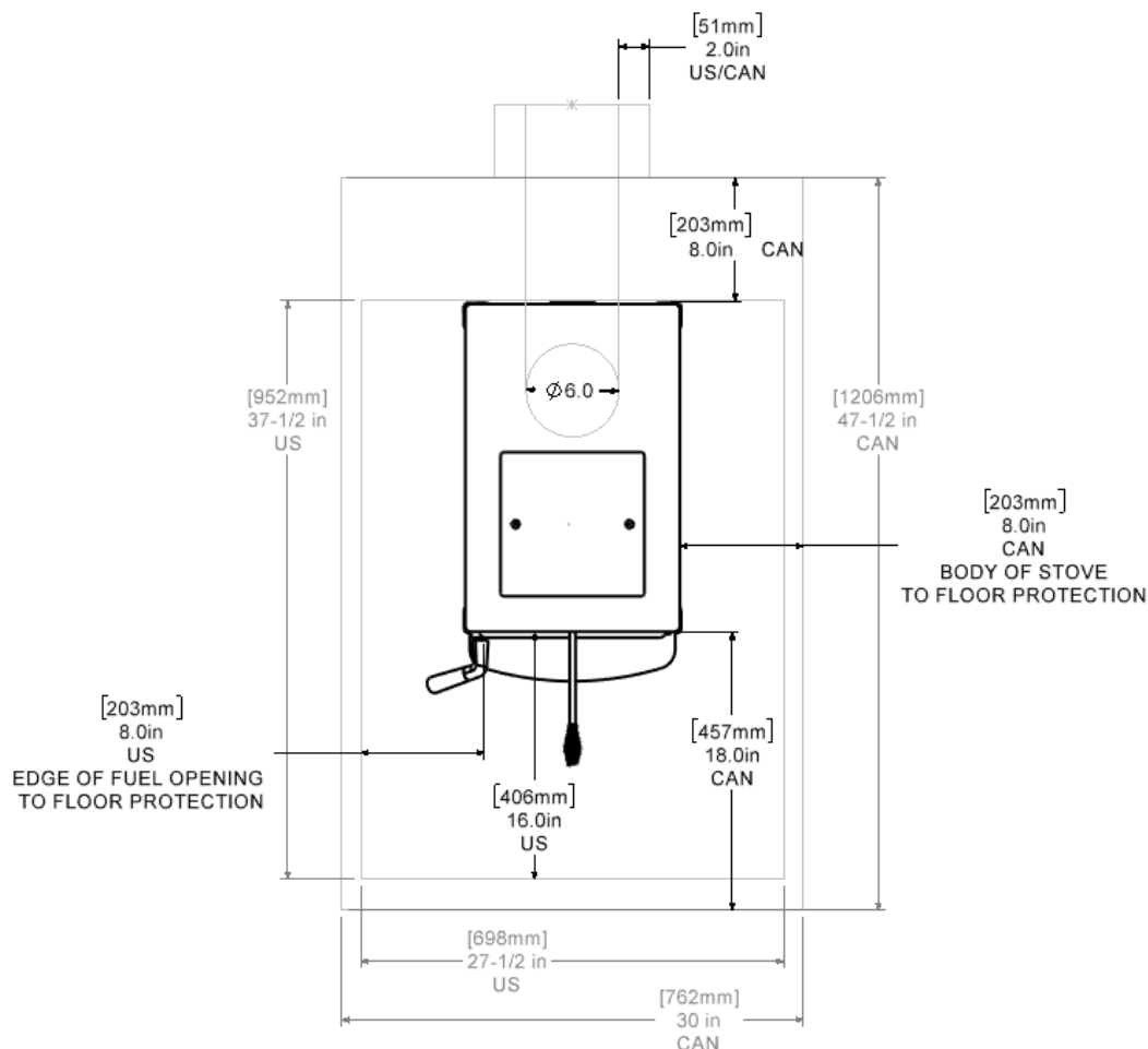
Figure 5 – Hearth Dimensions
