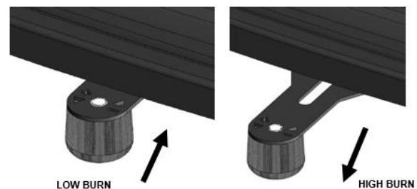
Figure 15 - Air Control
