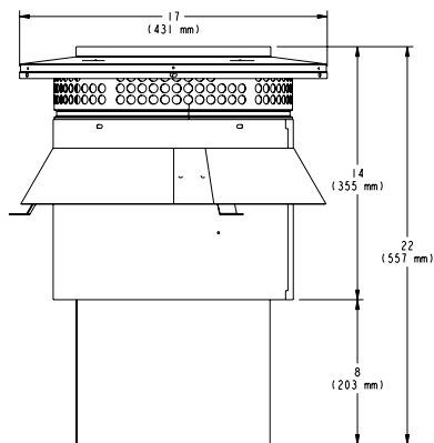
CB576 Chimney Joint Band
